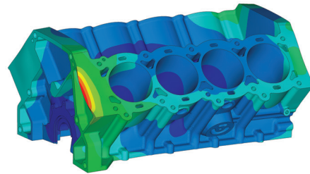
A static, linear structural analysis of an engine block without the internal components. Model Characteristics: PCG solver, symmetric matrix, 14.2 million DOFs
