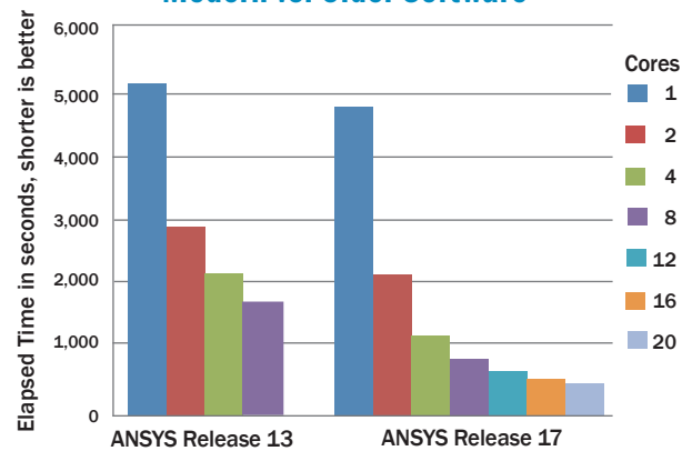
ANSYS release 17 running on a current Dell workstation showed significant reductions in solver times on a linear structural analysis of an engine block as core counts increased.
